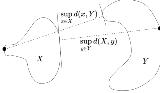
FIGURE 1.5. Hausdorff distance.
