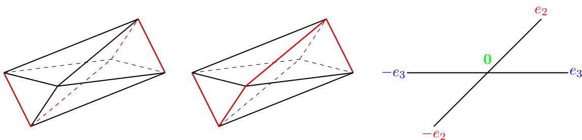
FIGURE 3.1. There are precisely two incoherent monotone paths on the octahedron, which are picture in the left and middle of the figure. The obstruction is pictured on the right, since both paths contain -e_3, -e_2, e_2 , and e_3 .
