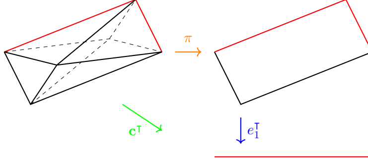
FIGURE A.2. Depicted is a description of coherence in terms of a commutative diagram. Namely, the path depicted is coherent, since it arises as the pre-image of the upper path on a polygon \pi(P) such that e_1^\top \pi = \mathbf{c}^\top . The coherent monotone path, the upper on the polygon, and the interval from \mathbf{c}^\top P are all highlighted in red to emphasize the correspondence between them.
