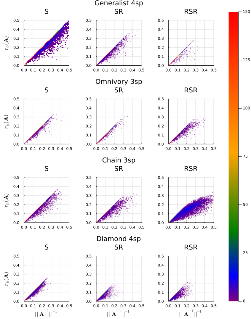
FIGURE 5.11. This figure gives a frequency 2D histogram the real distance to instability ( r_{\mathbb{R}}(\mathbf{A}) ) vs the distance to singularity |\mathbf{A}^{-1}|^{-1} for several module structures. For nearly normal systems, these points should be near the y = x line, however, it is clear that even stable, nonreactive systems can be closer to instability than their spectrum suggests. All of these parameter sets are of the same size, each histogram represents a subset of 10,000 points.
