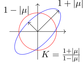
FIGURE 2.2. Quasiconformal maps
