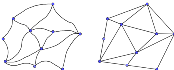
FIGURE 3.2. Tutte’s embedding
